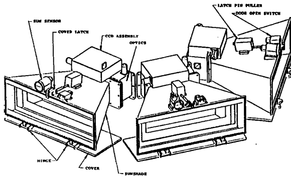
Fig. 3. Layout of the proposed SMEI.
