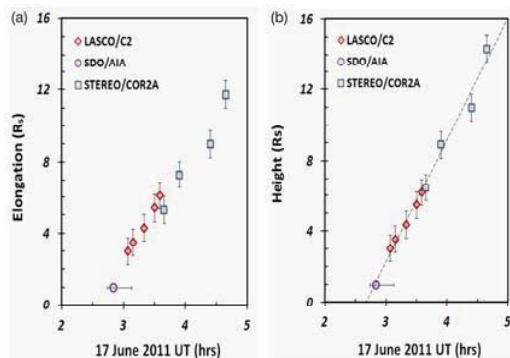
FIGURE 4. The height-time plots of the outward motion of the jet shown in Figure 3a. The structure’s radial extent is measured; the vertical bars indicate the central extent of the outward moving structure, and the horizontal bar on the jet response at 1 Rs indicates the duration of the brightest portion of the jet ejecta observed in AIA images. (a) outward progression of the jet response on the sky plane. (b) outward progression in height (the distance from the center of the Sun).
