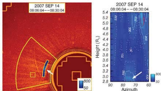
FIGURE 2. LASCO C2 background subtracted image overplotted with the blue-colored speed results at 2.8Rs obtained from the 2D cross-correlation (left-panel). The speed summary plot at different heights and azimuth angles is presented in the right panel. The jet response is marked by the white arrow.
