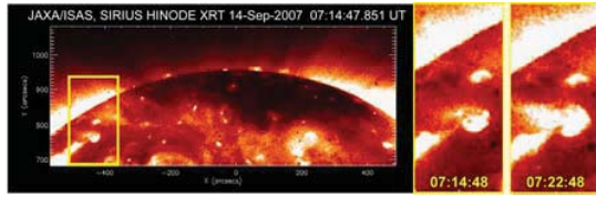
FIGURE 1. Hinode XRT data showing the north solar pole region, imaged in campaign mode in September 2007. The two right panels show an enlarged region of the jet response on 14 September 2007 at the time indicated (at 56°E, 57°N in ecliptic coordinates relative to the Sun center observed from Earth). The jet ejecta response moves away from the Sun non-radially and eastward relative to its solar surface location.
