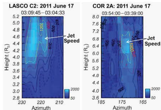
FIGURE 5. Synopsis of the speed measured with height in the regions surrounding the locations of the jet responses observed in two successive coronagraph images. The arrow locates the jet response in the two measurement sets. The analysis program shows that the jet response moves outward at speeds of >1200 \text{ km s}^{-1} . (left) LASCO C2 synopsis. Other fast outward motions are recorded near the jet response. (right) COR 2A synopsis. The fast region extent is \sim 1.5 Rs.
