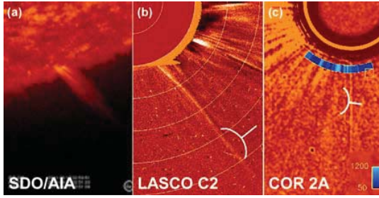
FIGURE 3. (a) SDO AIA jet observed during the HOP-187 period at \sim 02:50 UT on 17 June 2011. (b) LASCO C2 coronagraph enhanced image of the jet response. The bracket shows the location of the jet feature that is associated with the most intense portion of the jet response in SDO AIA images. (c) COR 2A (STEREO ahead spacecraft) coronagraph image of the jet response. The bracket shows the structure that is associated with the same feature observed in the AIA images. Superimposed on this image is the 2D cross correlation velocity determination provided at 3.6 Rs from this and the following coronagraph image. A high velocity region (see light blue band) is observed associated with the highlighted structure.
