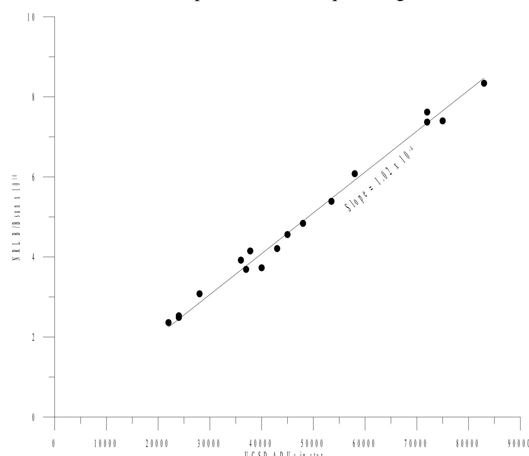
Fig. 2. Calculated expected B_{\text{star}}/B_{\text{sun}} versus total observed ADUs from SMEI.
