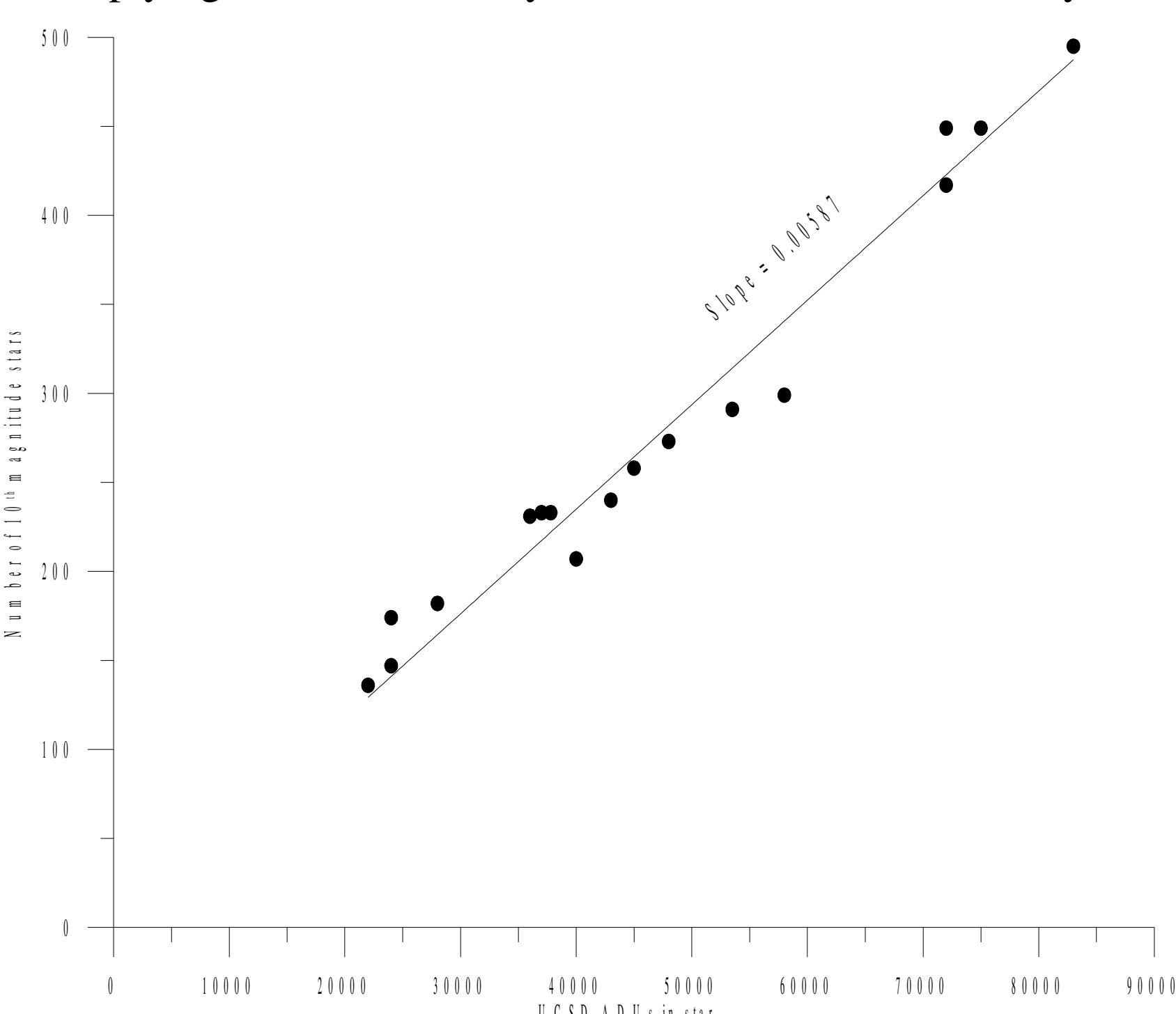
Fig. 1. Calculated expected equivalent number of 10 th magnitude stars versus total observed ADUs for SMEI. The SMEI data are averaged over four years for each of the seventeen stars.
